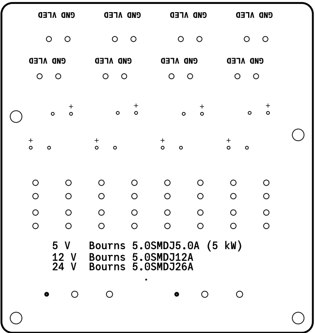
View from Bottom side (Scale 1:1)
