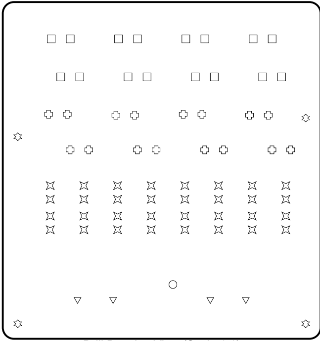
Drill Drawing View (Scale 1:1)
