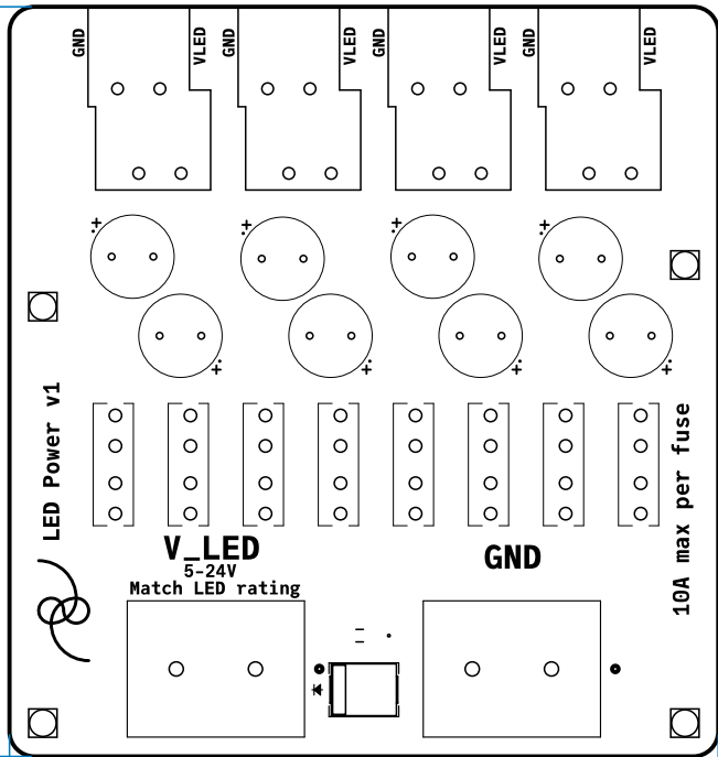
View from Top side (Scale 1:1)
