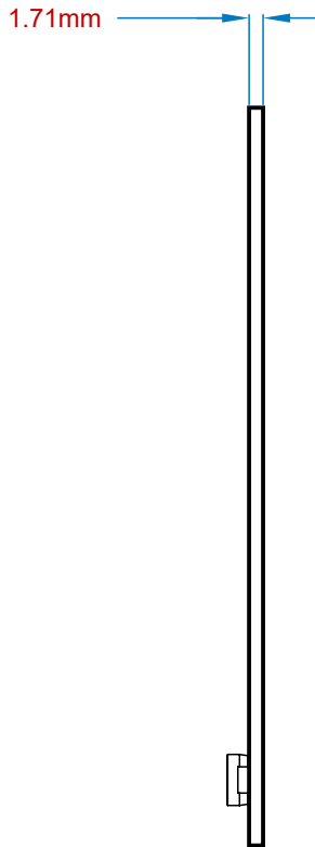
View from Right side (Scale 1:1)
